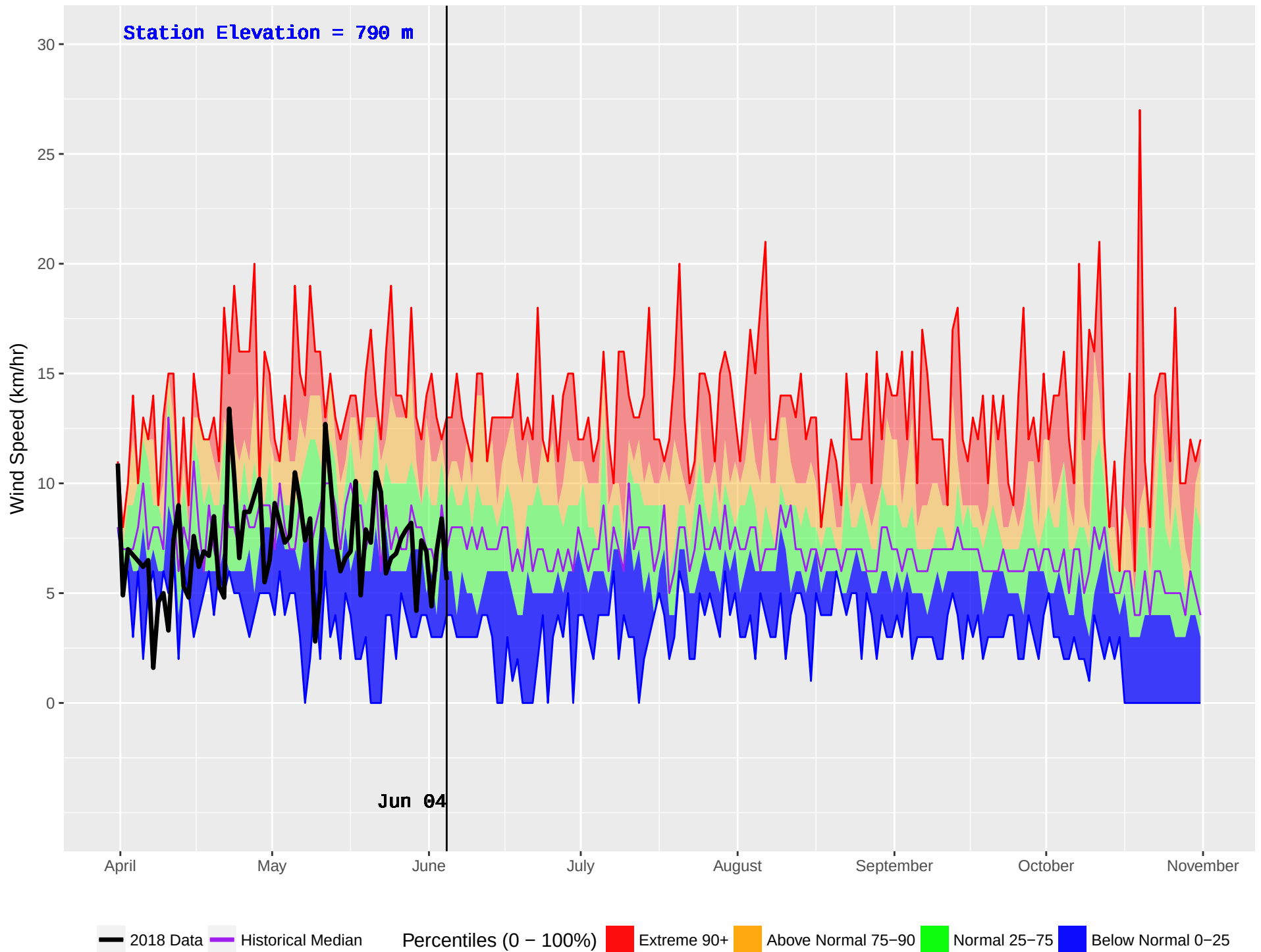
FALLS CREEK (383) : Historical (2002–2016) and Current (2018) Noon Wind Speed
