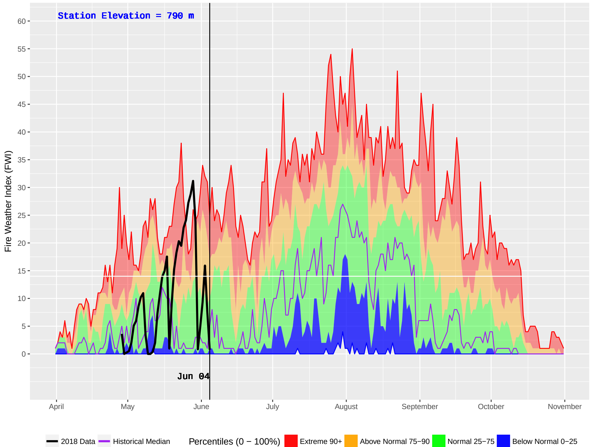
FALLS CREEK (383) : Historical (2002–2016) and Current (2018) Noon Fire Weather Index (FWI)
