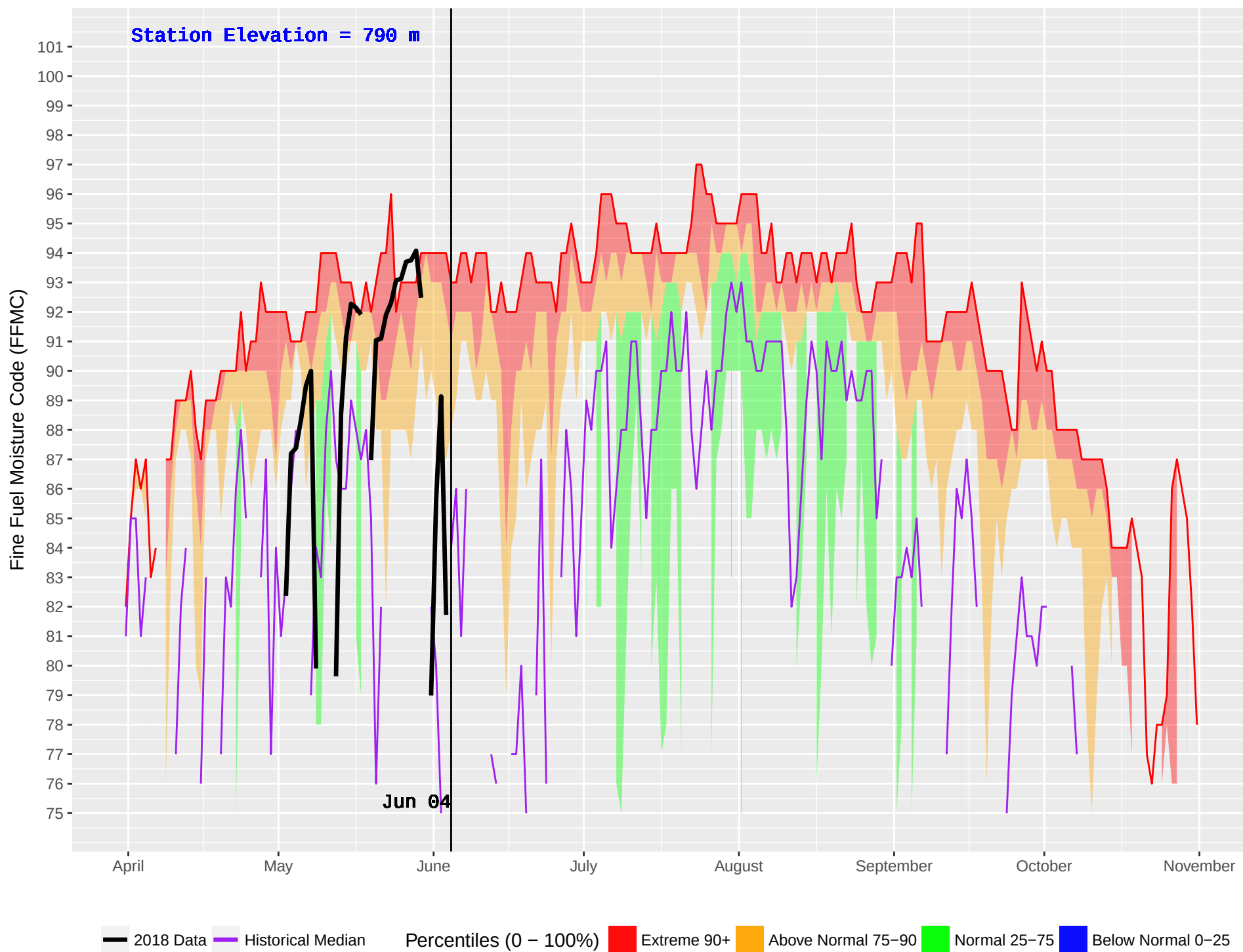
FALLS CREEK (383) : Historical (2002–2016) and Current (2018) Noon Fine Fuel Moisture Code (FFMC)
